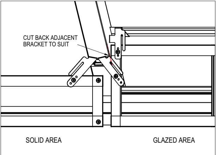
Typical Hip
