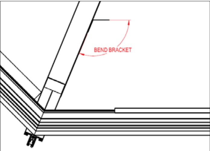
Hip position
