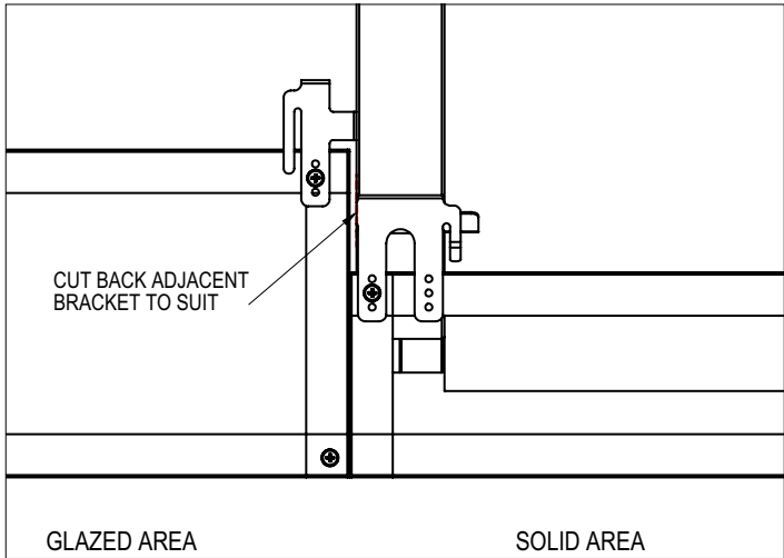
Typical Transom.
