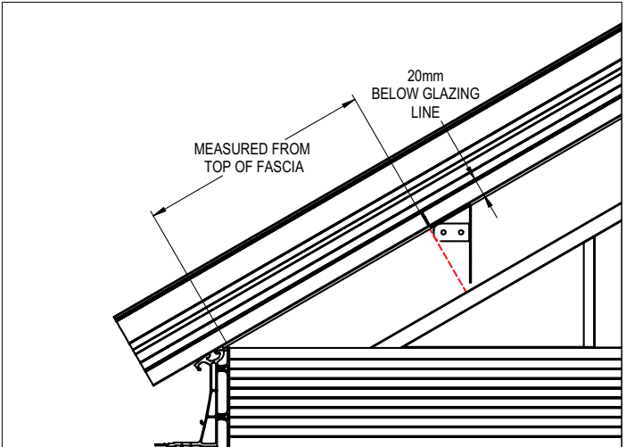
Gable position
