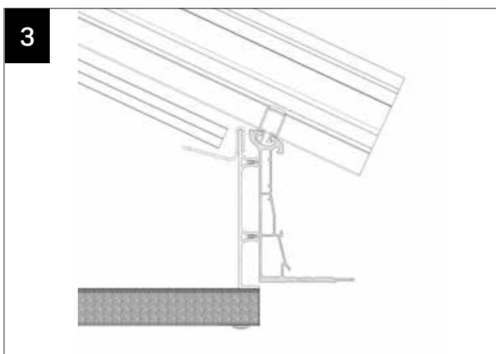
BELOW FASCIA
