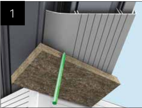
Cut a 200mm length of valley undercladding. This will act as a template for the bottom scribe. Use a 'straight edge' placed tight to the eaves fascia, then mark and cut.
