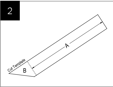
Measure dimension A then add B for overall length. Mark and cut the claddings for both left and right side. Push fit the claddings into position.
