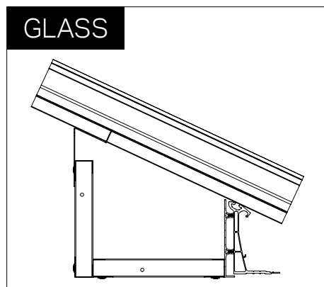
Pelmet position
